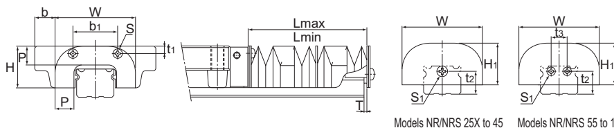
Models NR/NRS 25X to 45
